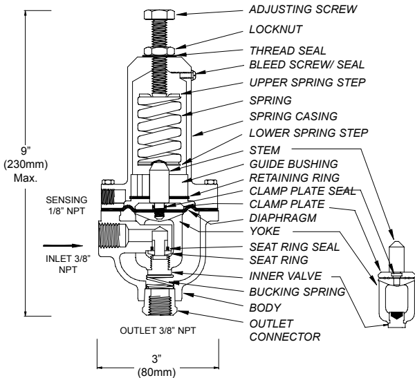
SCHEMATIC A0709D
