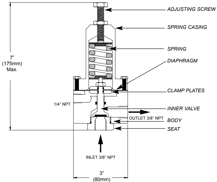
SCHEMATIC A0781A
