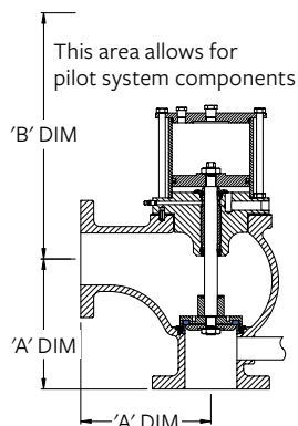
PNEUMATIC (ALL PRESSURE RANGES PLUS EXCESSIVE PRESSURES)
