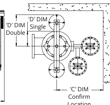
ASSEMBLY CLEARANCE (APPLICABLE TO ALL MODELS)
