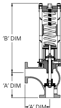
SINGLE SPRING STACK (LOWER PRESSURE RANGES)
